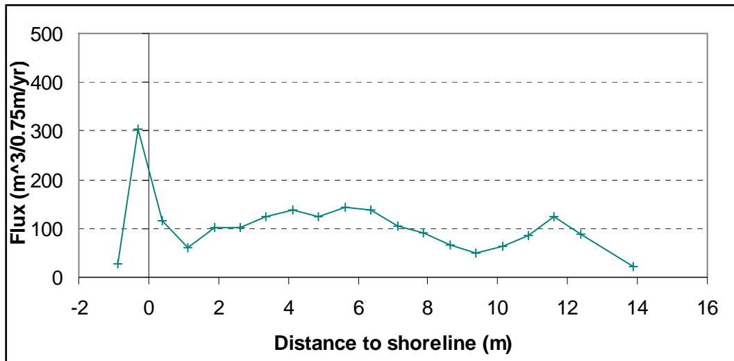
Figure 71. Cross-shore distribution of longshore sediment flux, T1C8.
