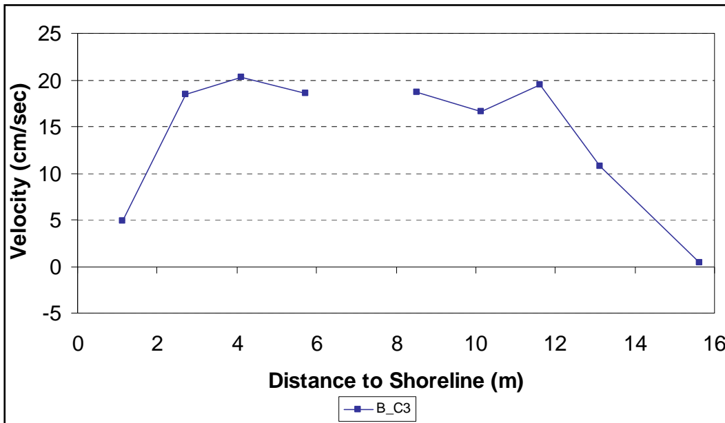
Figure 15. Cross-shore distribution of longshore current, B_C3.
