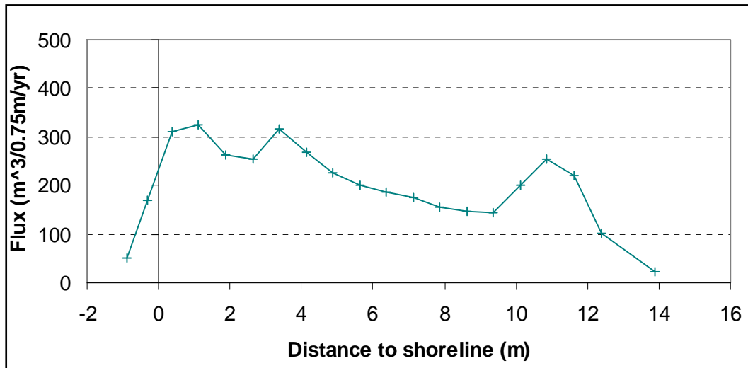
Figure 80. Cross-shore distribution of longshore sediment flux, T2C2.
