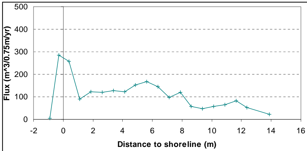
Figure 8. Cross-shore distribution of longshore sediment flux, B_C1.
