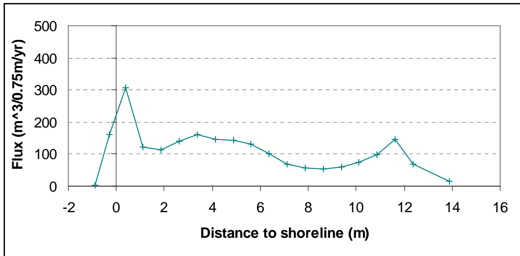
Figure 132. Cross-shore distribution of longshore sediment flux, T3C4.
