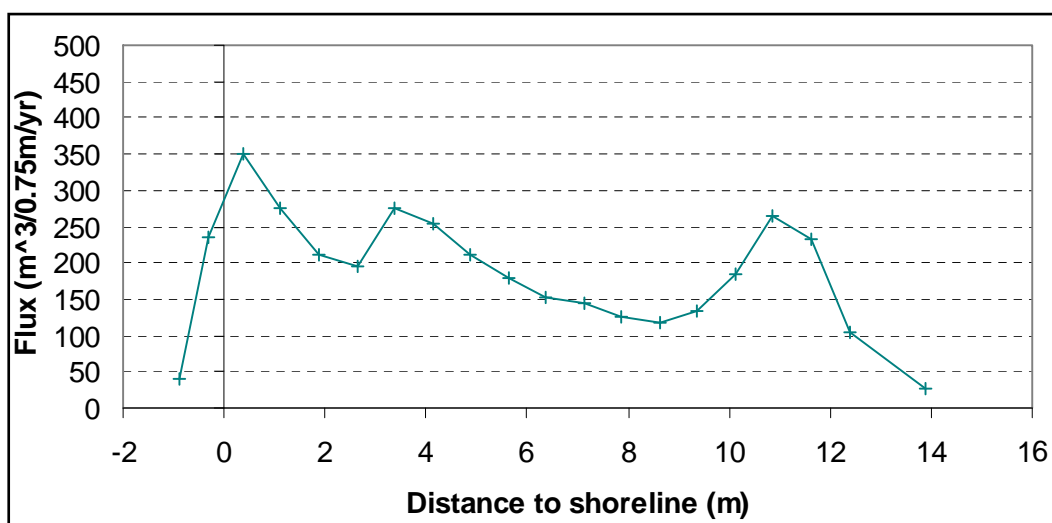
Figure 89. Cross-shore distribution of longshore sediment flux, T2C4.
