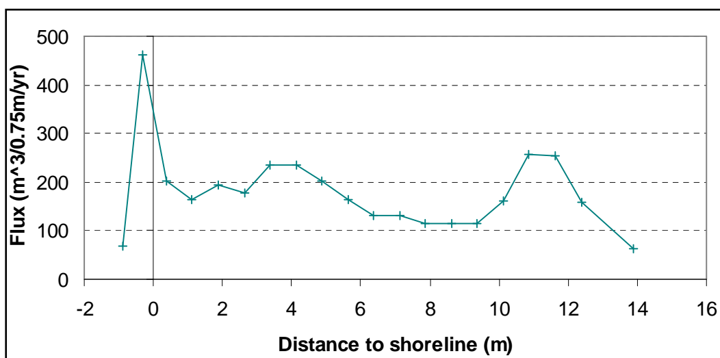
Figure 94. Cross-shore distribution of longshore sediment flux, T2C5.
