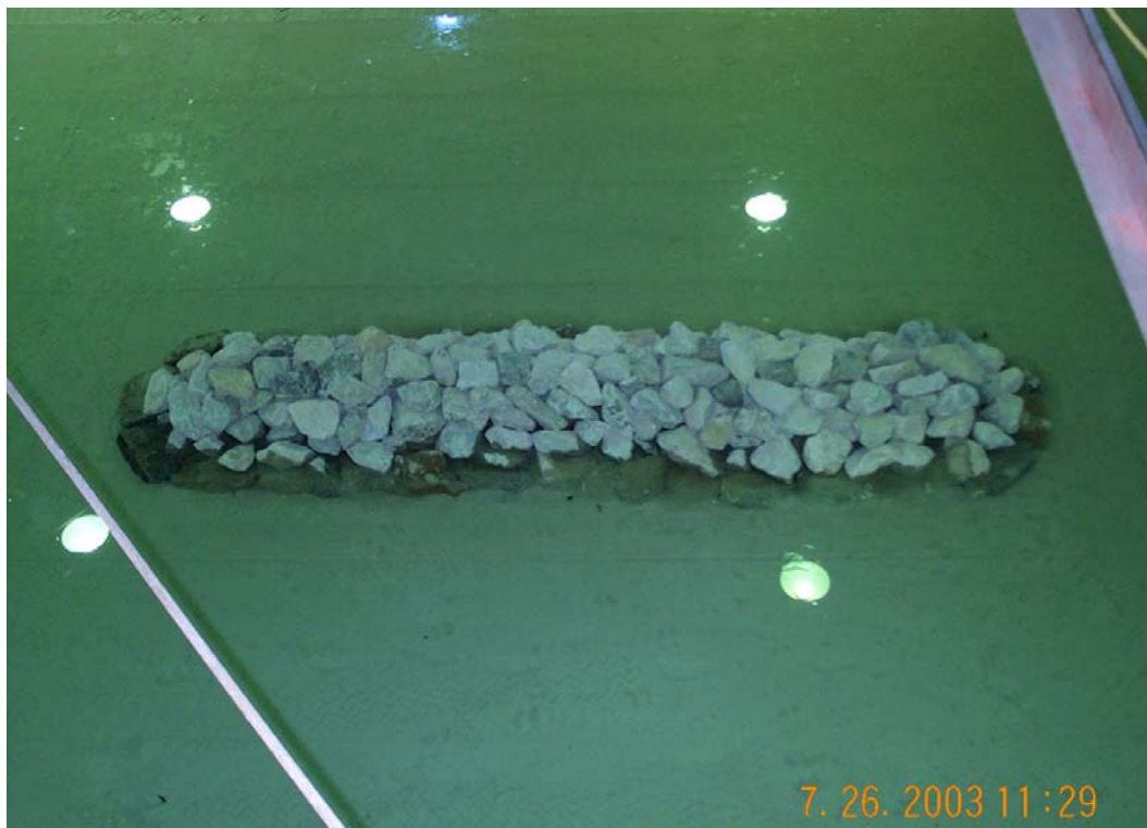
Figure 31. Breakwater structure in filled LSTF at operating water level.
