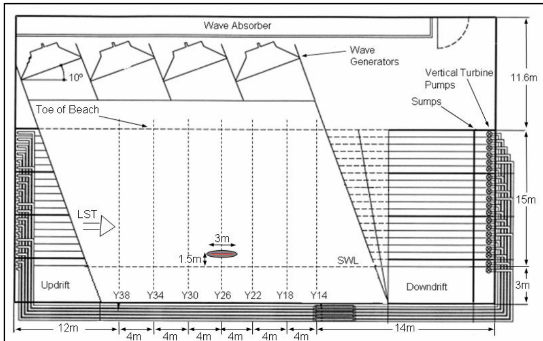
Figure 3. Nearshore breakwater layout within LSTF (Test 4).
