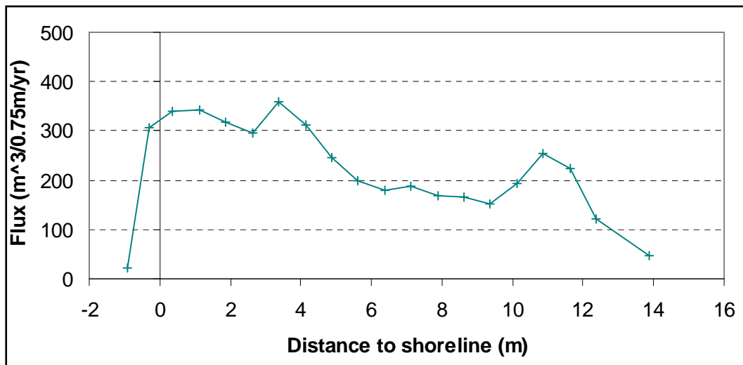
Figure 76. Cross-shore distribution of longshore sediment flux, T2C1.
