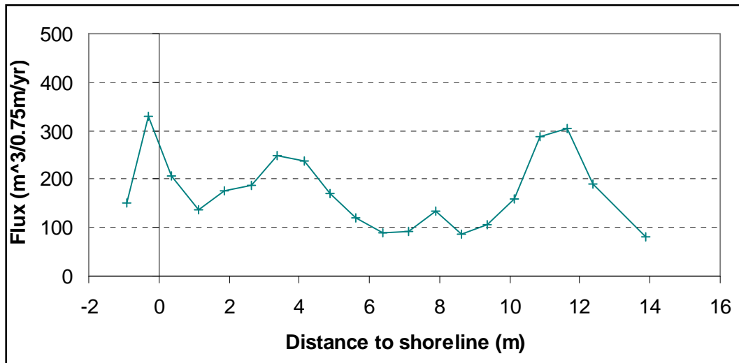
Figure 103. Cross-shore distribution of longshore sediment flux, T2C7.
