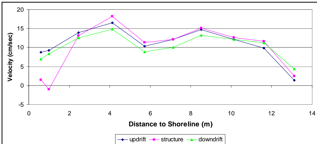
Figure 148. Cross-shore distribution of longshore current, T4C1.
