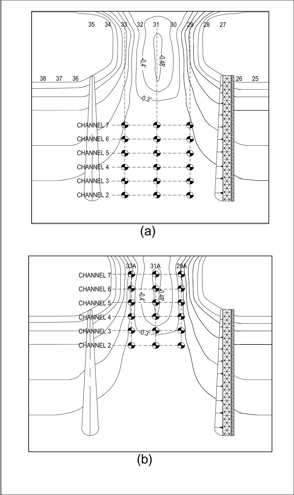
Figure 16. Wave gauge locations (a) in outer portion of channel and (b) inside portion. Range numbers shown at top of figure
