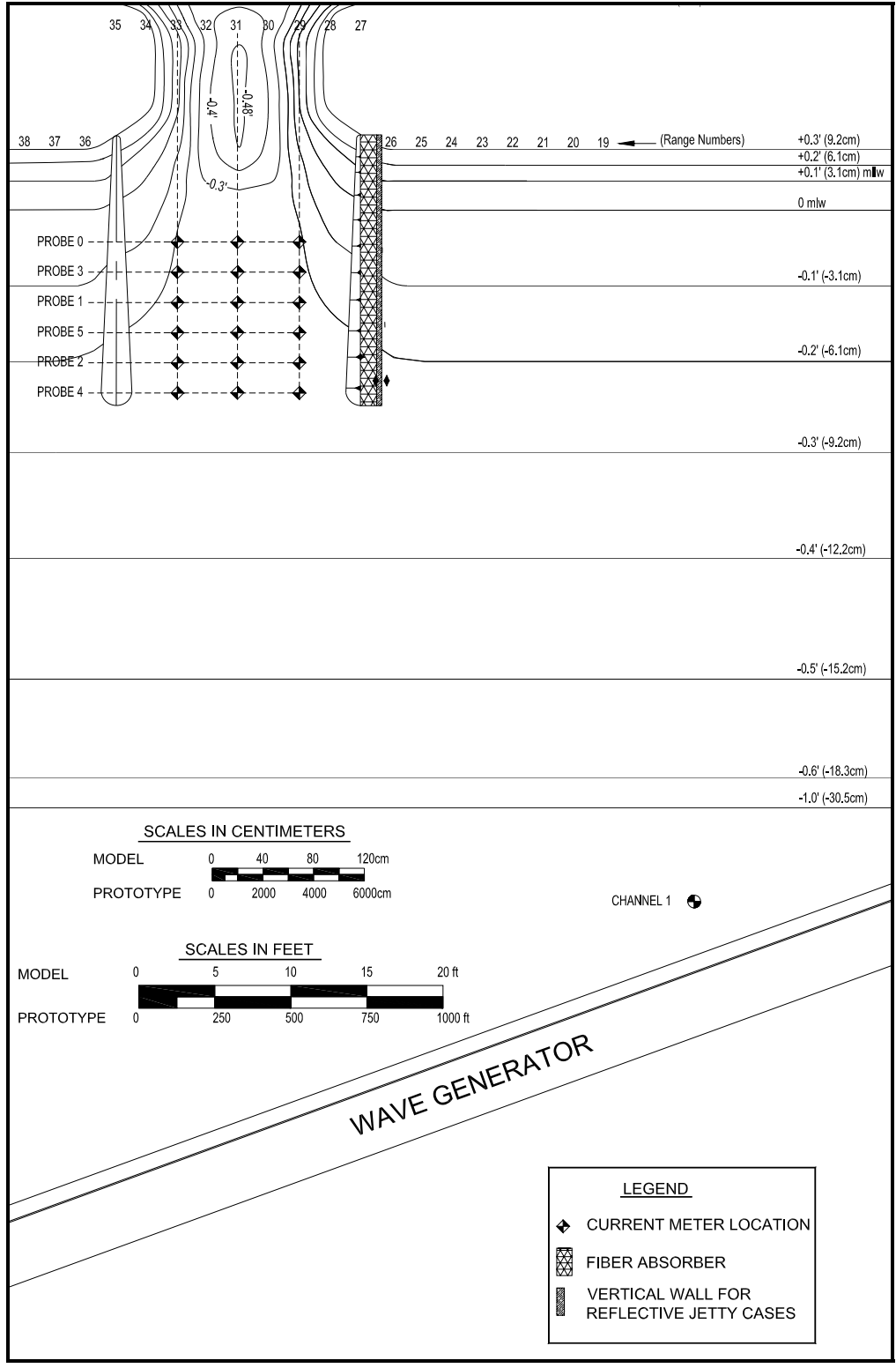
Figure A5. Current meter layout in outer channel for measurements conducted inside the inlet. Depth contours are shown in model scale units in feet (centimeters)
